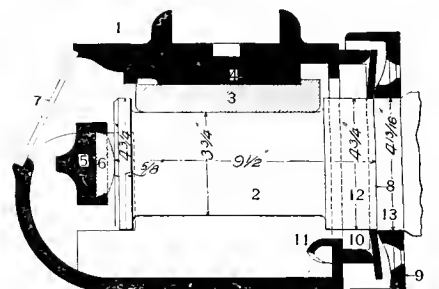
Fig. 5149. Applied to a Collared Journal. BOSTON & ALBANY RAILROAD. (350)
